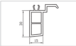
FBA 30 mm
